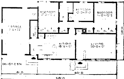
A SMALL HOUSE PLANNING BUREAU DESIGN NO. C-554
